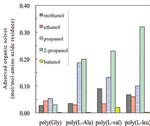
Fig. 2 Adsorption of each alcohol on each polypeptides at vapor pressure, 10kPa
